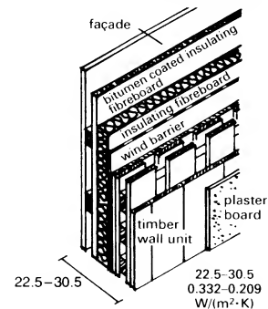
⑮ Variation of Lignotrend 22.5-30.5 0.332-0.209 W/(m 2 ·K)
